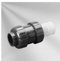
Fußventil S4 DN80 PVC grau PVC-U Klebemuffe d 4" ASTM PN6 EPDM EPDM Foot valve S4 DN80 PVC grey PVC-U solvent socket ends d 4" ASTM PN6 EPDM EPDM
